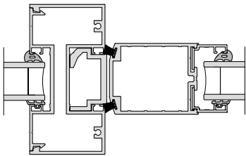
GT55 NI JAMB LOCKING STYLE
